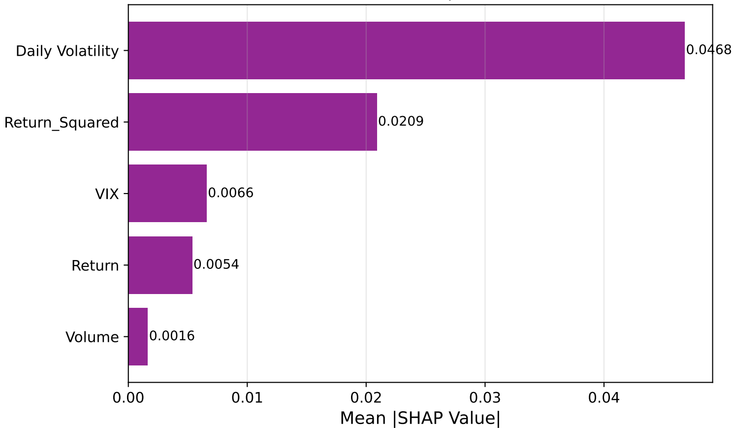
LSTM (VIX) — Feature Importance via SHAP
